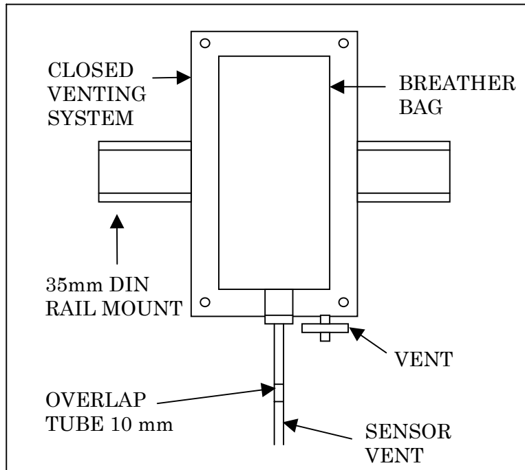
Figure 2. Venting System
